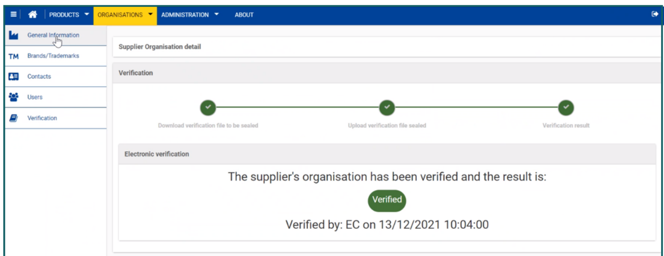
Figure 31: Successful Verification
