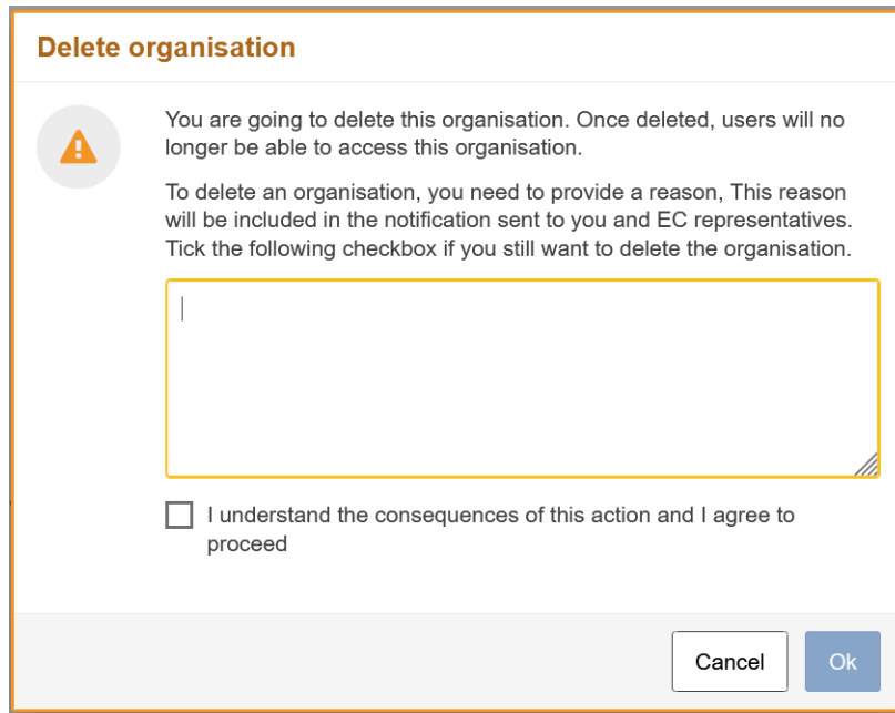
Figure 44 - Deletion confirmation
