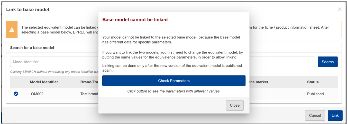
Figure 93 - Linking error
