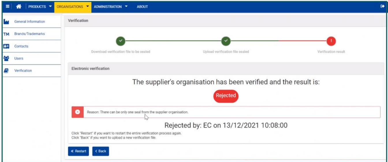
Figure 32: Unsuccessful Verification
