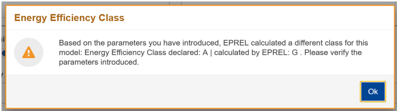
Figure 64 - Check warning
