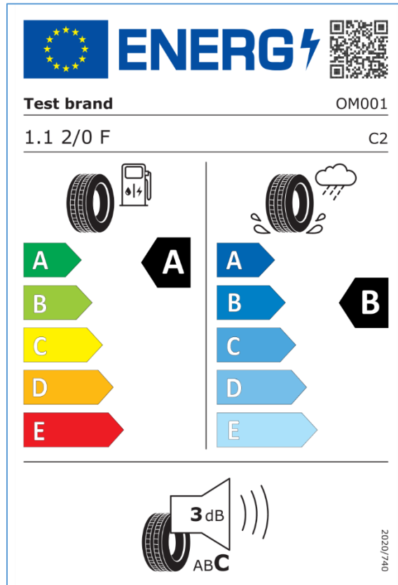
Figure 52 – Tyres label
