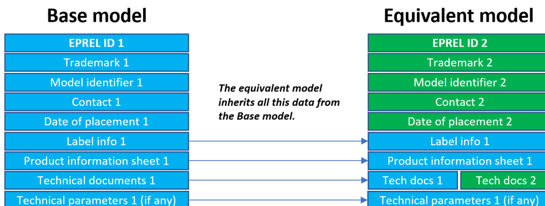
Figure 96 - Data linking
